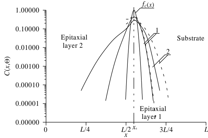
Fig.3b. Calculated distributions of implanted dopant in epitaxial layers of heterostructure. Solid lines are spatial distributions of implanted dopant in system of two epitaxial layers.
