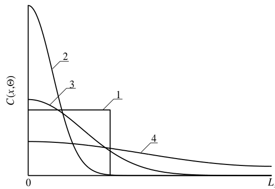
Fig.4a. Distributions of concentration of infused dopant in depth of heterostructure from Fig. 1 for different values of annealing time (curves 2-4) and idealized step-wise approximation (curve 1). Increasing of number of curve corresponds to increasing of annealing time
