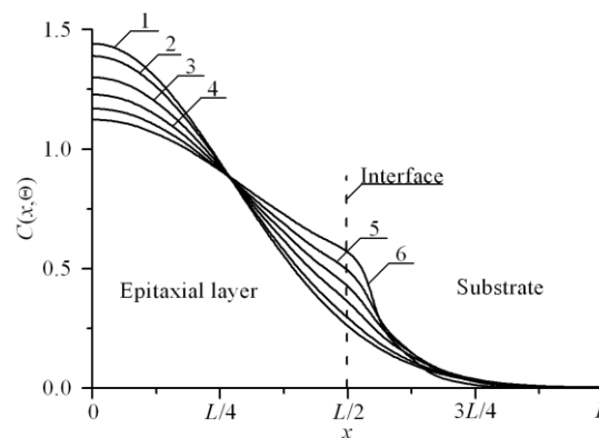
Fig. 2a. Dependences of concentration of dopant, infused in heterostructure from Figs. 1, on coordinate in direction, which is perpendicular to interface between epitaxial layer substrate.
